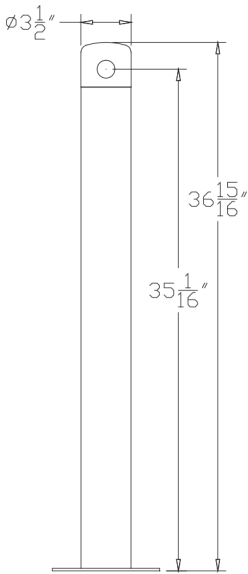
ELEVATION VIEW
