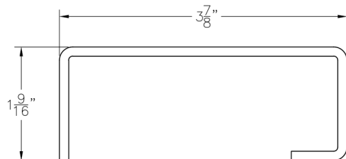
SP-212R FOR 2x12 REPLACEMENT PLANK 1 PAIR 18" LONG
