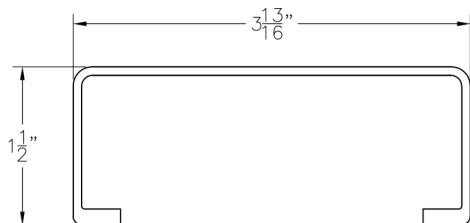
SP-208 FOR 2x8 PLANK 1 PAIR 18" LONG
