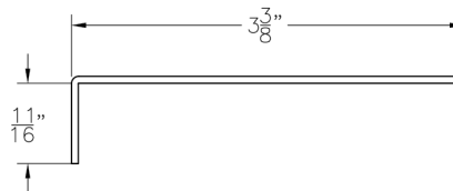
SP-108 FOR OLD STYLE 1x6 & 1x8 PLANK 1 PC. 12" LONG
