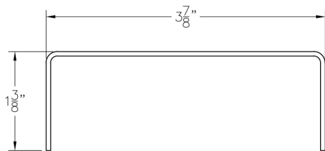
SP-205/207 FOR 2x5 & 2x7 PLANK 1 PC. 18" LONG
