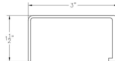
SP-210 FOR 2x10 & 2x12 PLANK 1 PAIR 18" LONG
